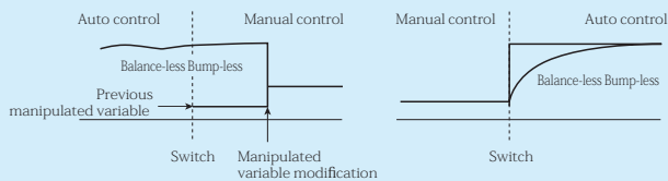
Balance-less Bump-less
